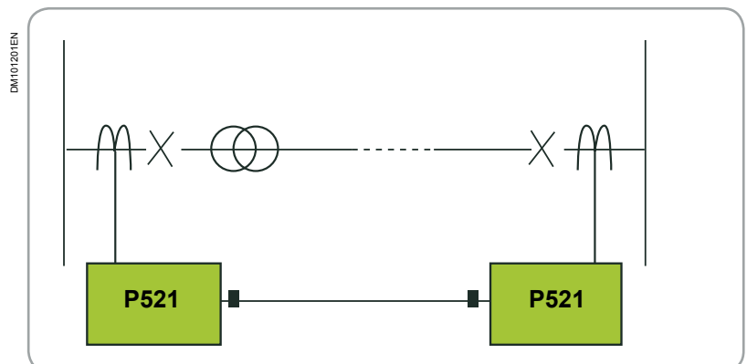
Fig.1 : P521 in-zone transformer application
