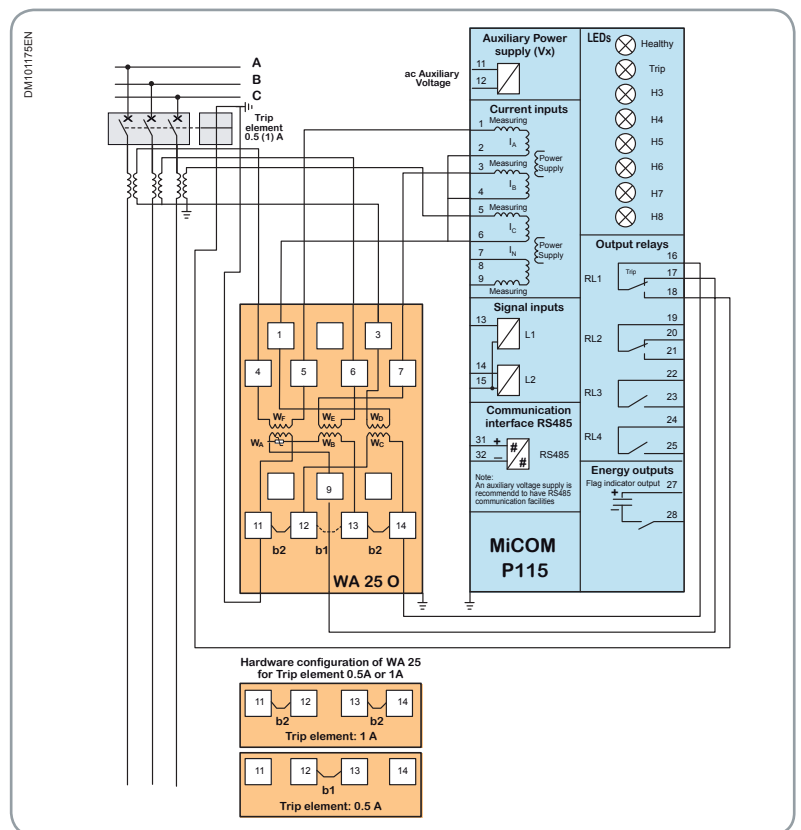
MiCOM P115 powered by a WA 25 O / 3 pole: Connection example for a P115 powered by a WA 25 O and with a 3 pole connection (A - B - C)
