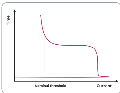
Cold-load characteristics
