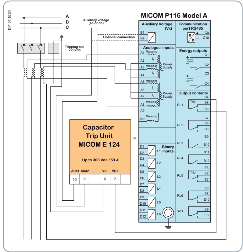
MiCOM P116 Model A powered by an E124:: Connection example for a P116 powered by an E124 and with a 4-pole connection (A-B-C-N). The earth input supplies the relay.
