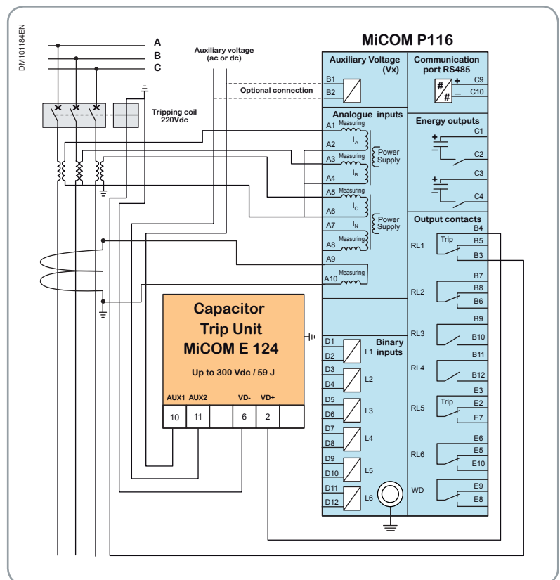
MiCOM P116 powered by an E124: Connection example for a P116 powered by an E124 and with a 4-pole connection (A-B-C-N). The P116 is not supplied via the earth input.
