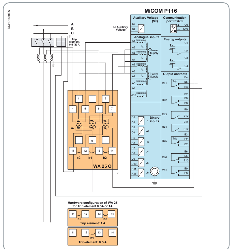
MiCOM P116 Model A powered by a WA 25 O: Connection example for a P116 Model A powered by a WA 25 O and with a 3-pole connection (A-B-C)
