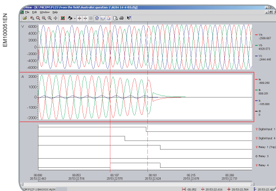
Example of disturbance record
