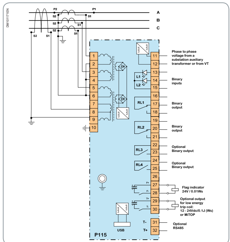
MiCOM P115: Typical 3 phase CTs + Core balanced CT connection. The P115 is not supplied via a Core Balance CT. An auxiliary voltage source should be connected to the 11-12 terminals in order to ensure that the P115 is supplied for earth fault currents below 0.2 In.
