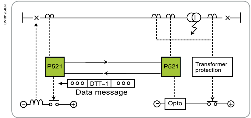
Fig.4 : Example Application of Direct Intertripping
