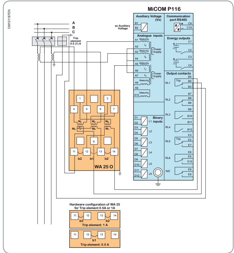
MiCOM P116 Model A powered by a WA 25 O: Connection example for a P116 Model A powered by a WA 25 O and with a 2-pole connection (A-C)
