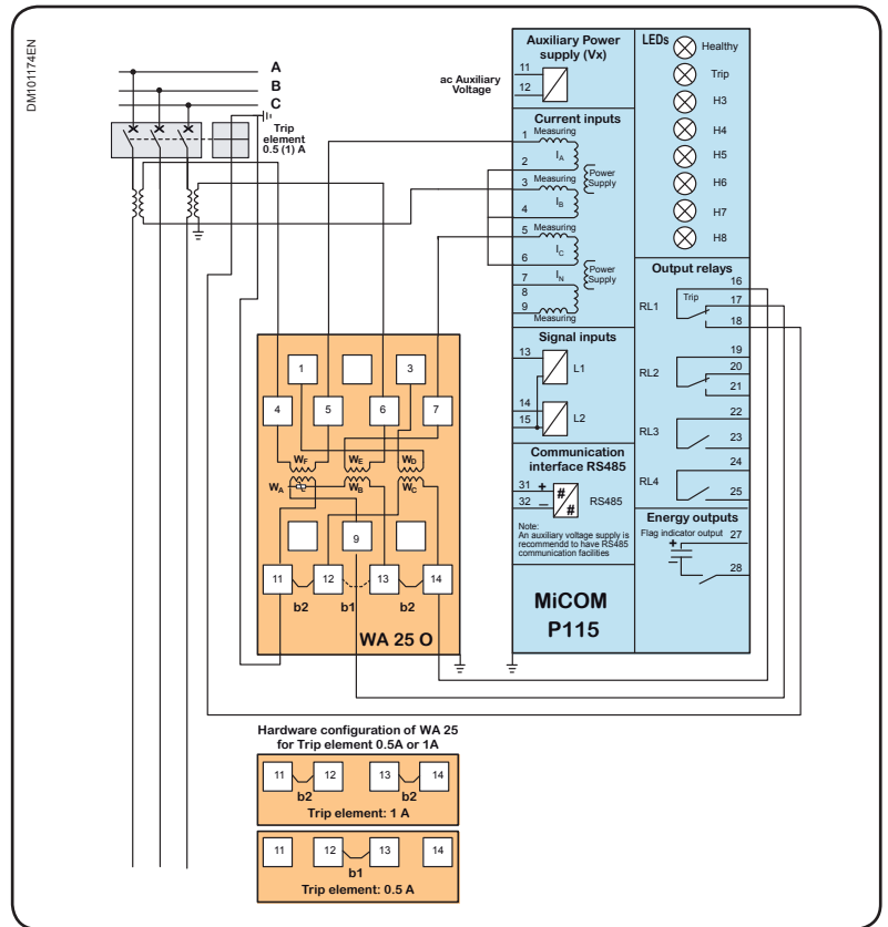
MiCOM P115 powered by a WA 25 O / 2 pole: Connection example for a P115 powered by a WA 25 O and with a 2 pole connection (A - C)
