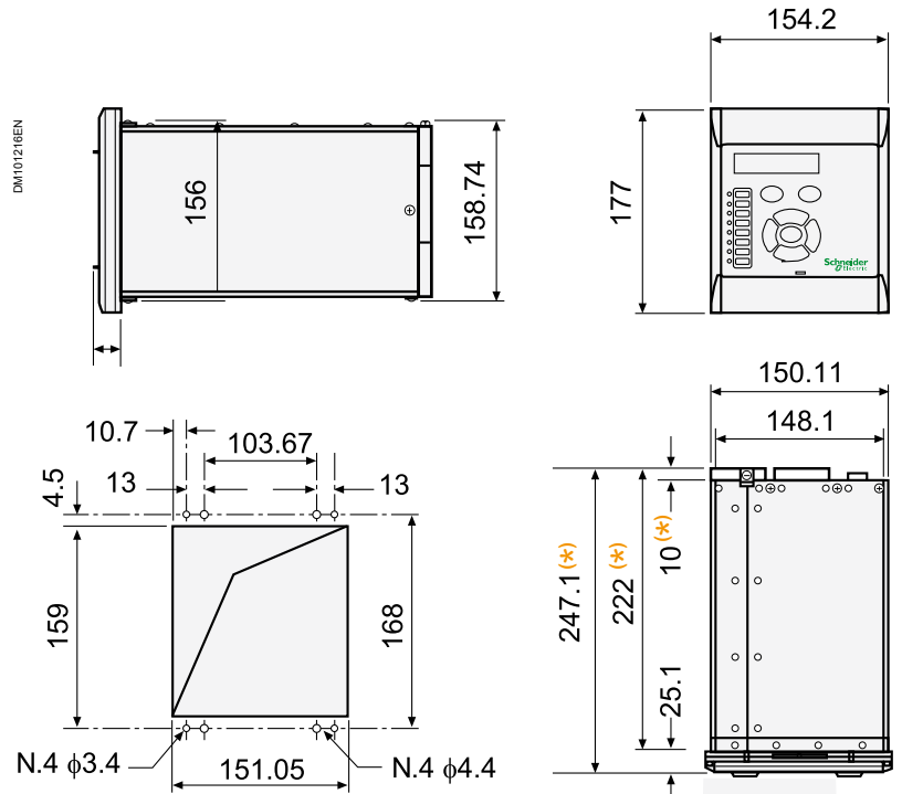
All dimensions in mm
