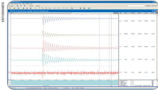
WaveWin – Data Analyzer Software
