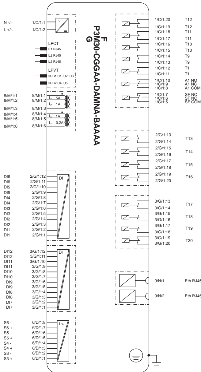
Figure 12 - P3F30 and P3M30 block diagram – LPIT
