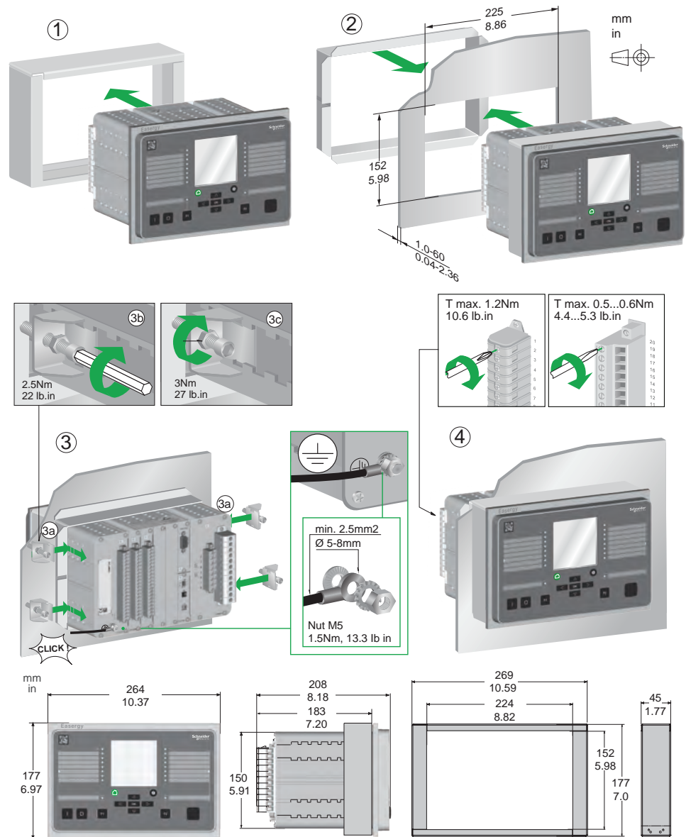
Figure 17 - Projection mounting
