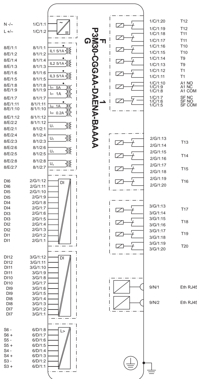
Figure 11 - Typical block diagram for P3F30, P3M30 and P3G30 relays
