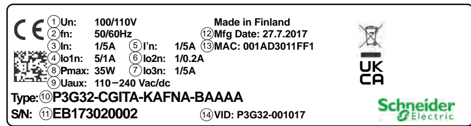
Figure 1 - Serial number label
