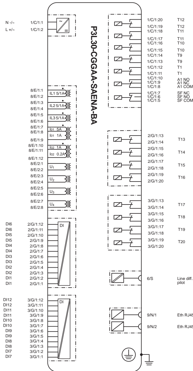
Figure 13 - Typical block diagram for P3L30 relay
