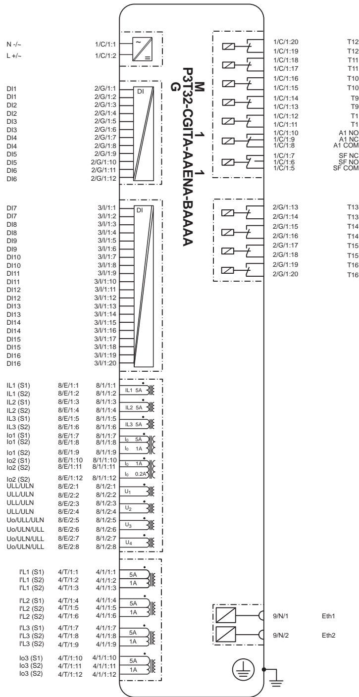
Figure 14 - Typical block diagram for P3M32, P3T32 and P3G32 relays
